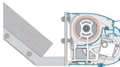
Rafter fixed With 10 or 22 Degree Rafter Bracket
