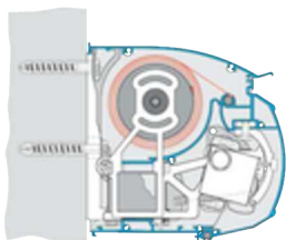
Wall fixed With Wall bracket
